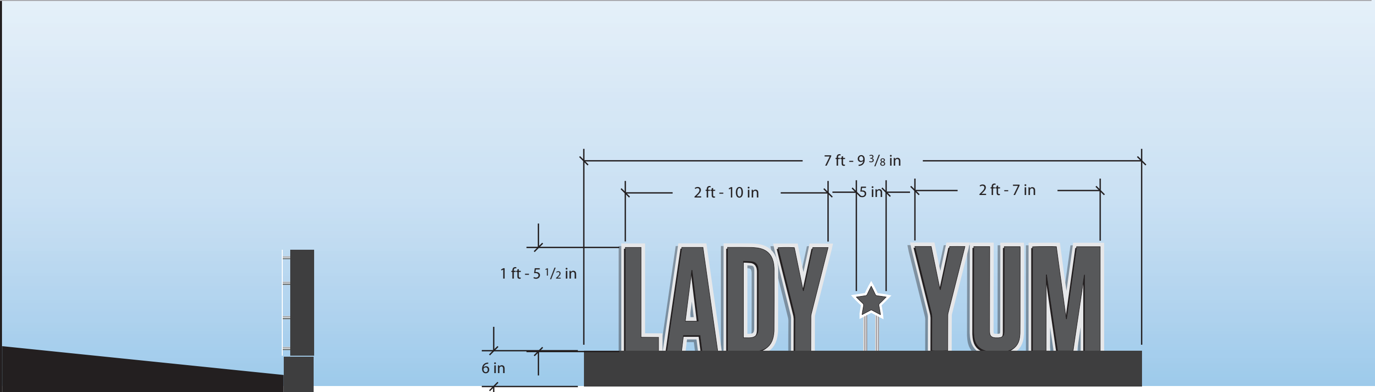
Side View Scale: 3/4" = 1'-0"
