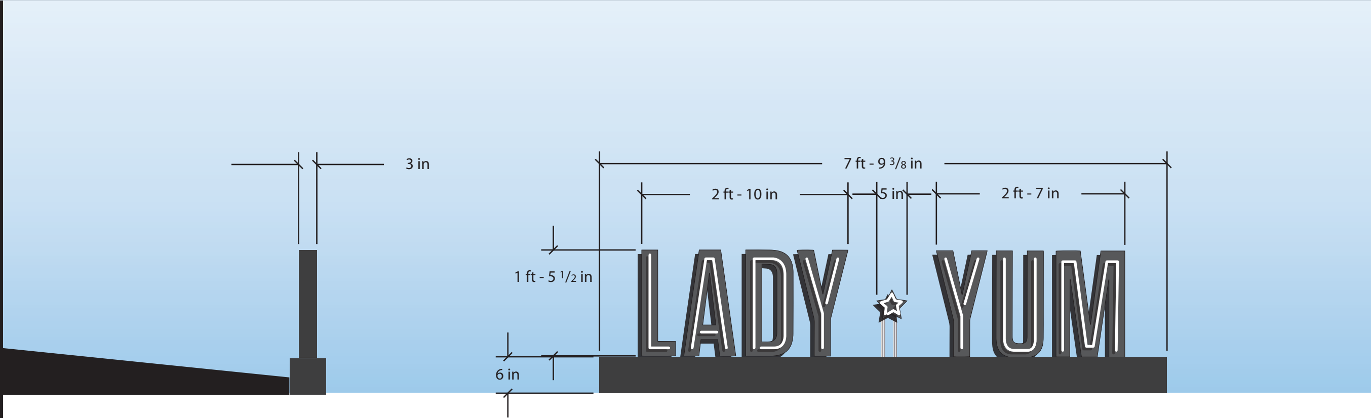
Side View Scale: 3/4"=1'-0"
