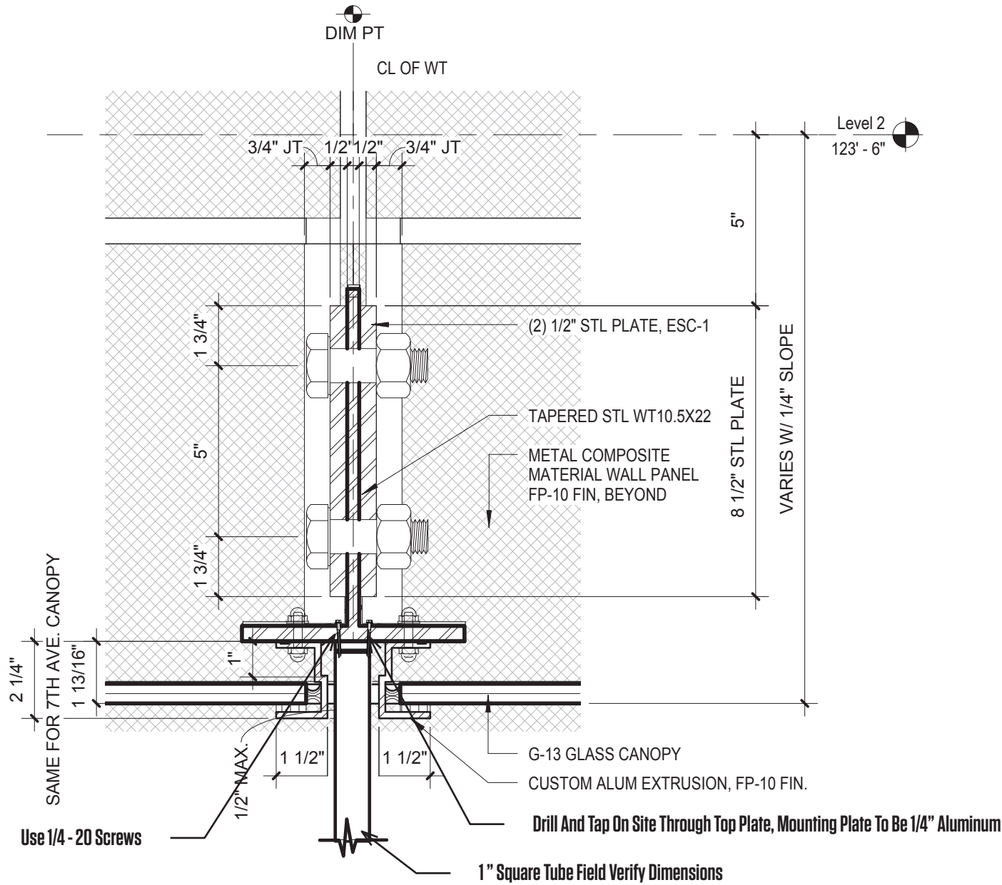
ELEVATION DETAIL OF CANOPY WT@ KNIFE PLATE BLADE SIGN MOUNTING DETAIL 3" = 1'-0"
